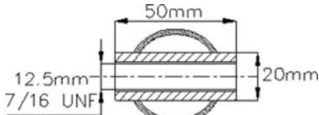
Dessin / Drawing 253-67
